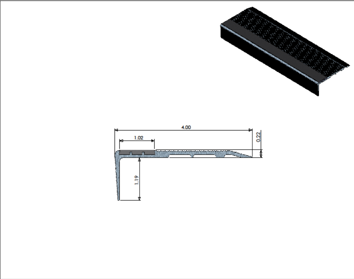
Metal Stair Tread Nosing Diagram (not to scale)
